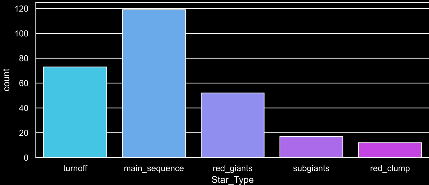
Field [103] Count plot of Star Type
