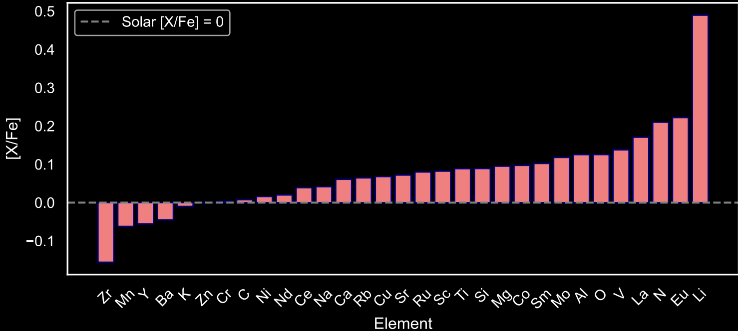
Abundance Pattern for GALAH Star Field [103] (N=273)
