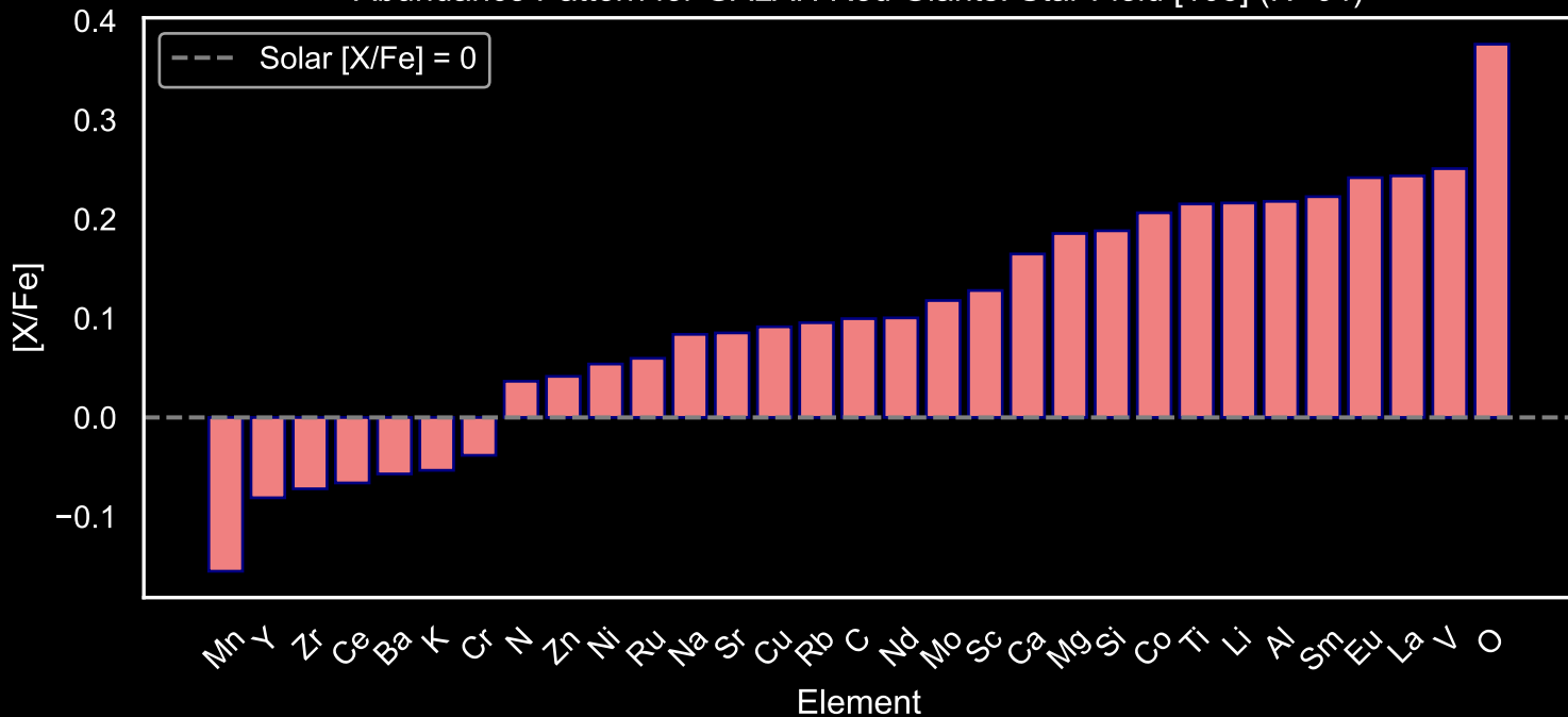
Abundance Pattern for GALAH Red Giants: Star Field [103] (N=64)
