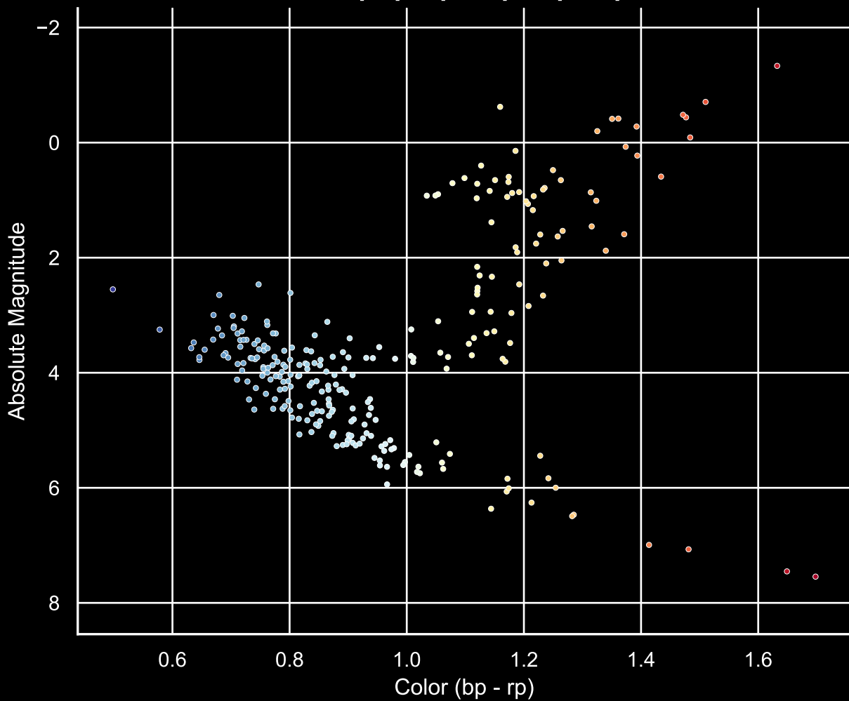
GALAH Hertzsprung-Russell Diagram Field [103] Ra [319.82] Dec [-24.22]
