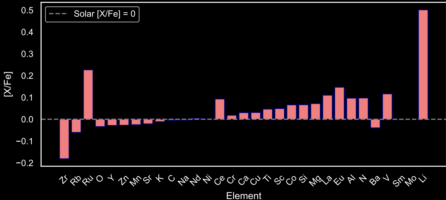
Abundance Pattern for GALAH Main Sequence Stars: Star Field [103] (N=119)
